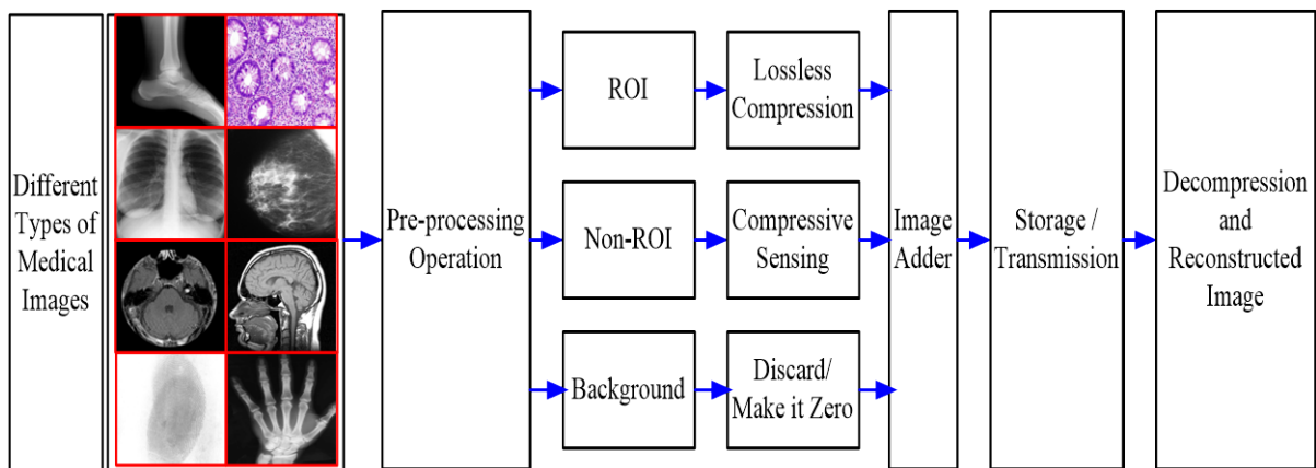
Figure 1. Architecture of the proposed MICCS method
