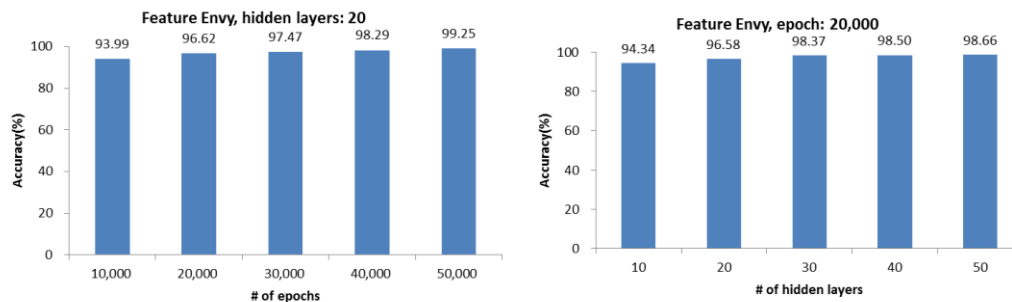
Figure 8. Accuracy of the Network Model when Detecting the Feature Envy Code Smell
