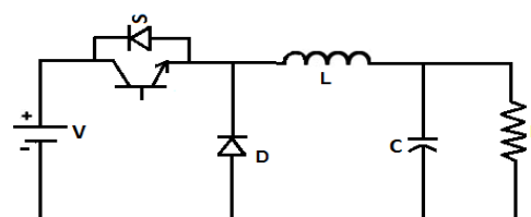
Figure 6. Circuit diagram of buck converter
