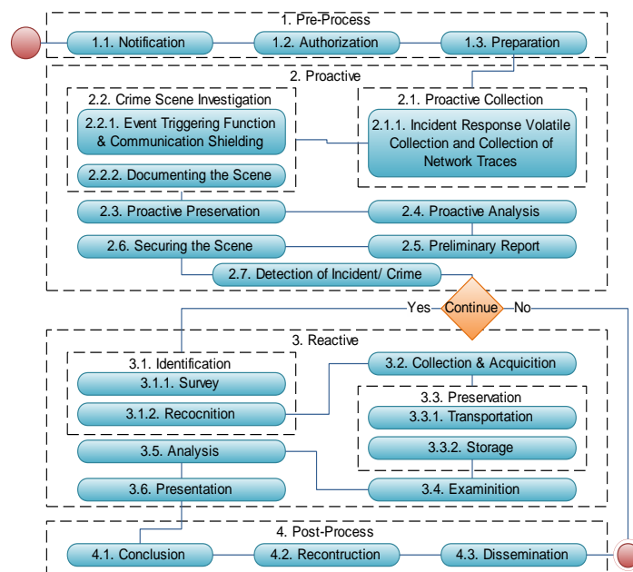
Figure 1. IDFIF model [7-8]
