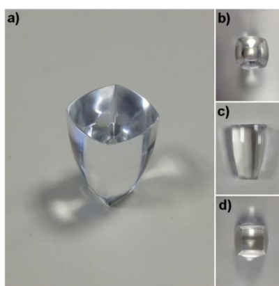
Figure 1. The RACPC prototype fabricated for experimental purposes, (a) the isometric view; (b) the top view; (c) the side view, and (d) the bottom view of the concentrator
