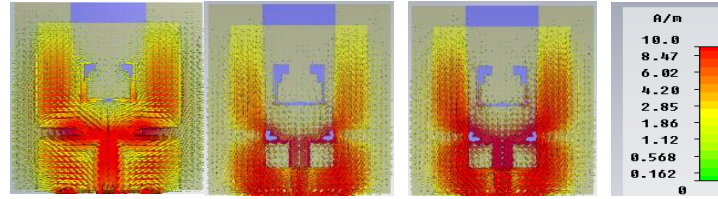
Figure 7. Simulated Surface current distribution of the final proposed antenna at (a) 0.9 GHz, (b) 1GHz and (c) 1.1GHz
