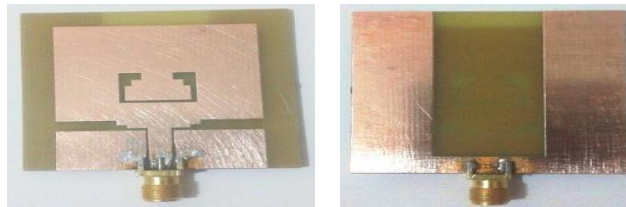
Figure 8. The fabricated antenna structure
