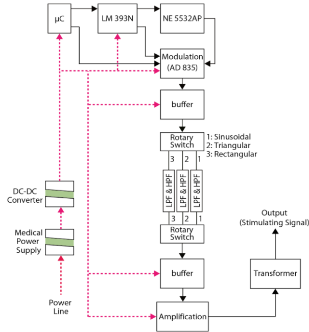
Figure 1. Functional Electrical Stimulator Architecture is Shown. HPF: High Pass Filter, LPF: Low Pass Filter
