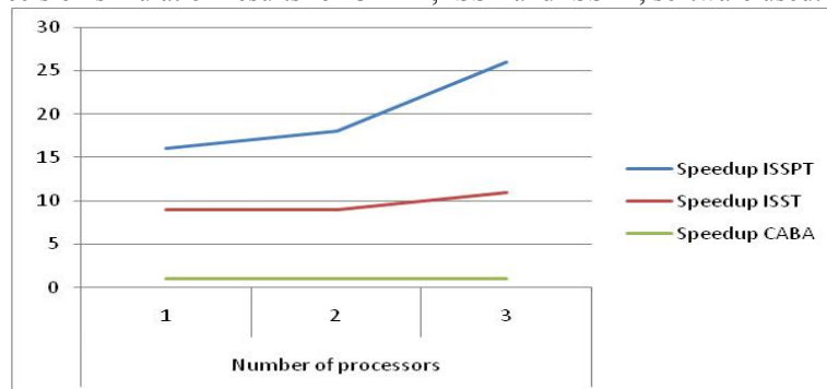
Figure 9. Speedup simulation results for CABA, ISST and ISSPT, software used: JPEG Encoder
