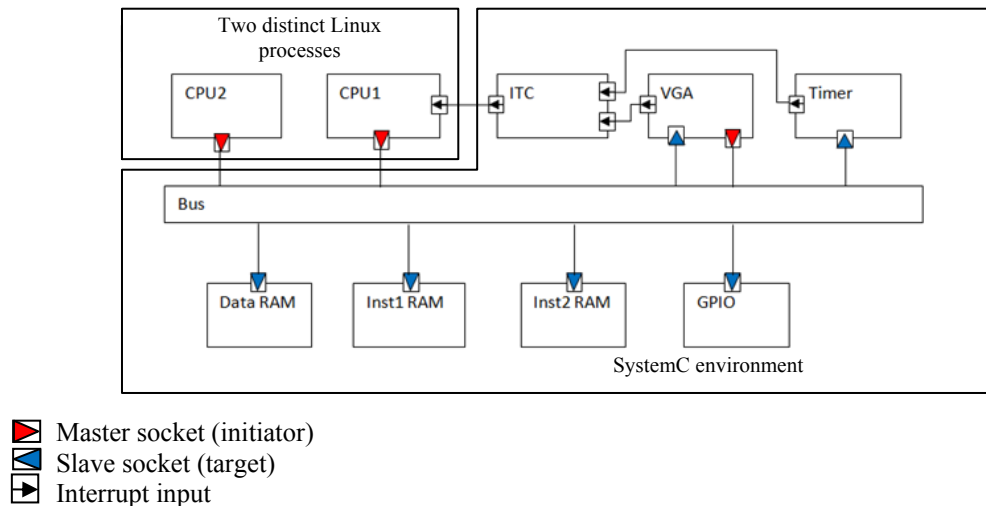
Figure 2. Platform architecture with 2 processors
