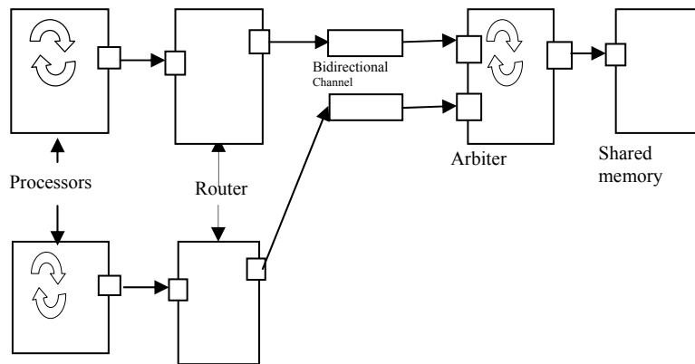
Figure 5. Crossbar implementation
