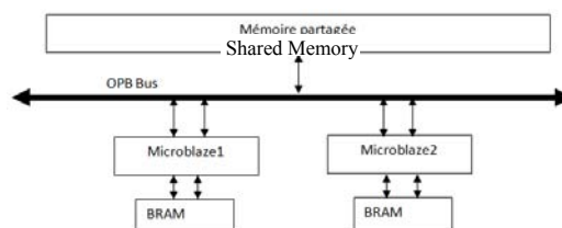
Figure 1. Multi-MicroBlaze basic architecture
