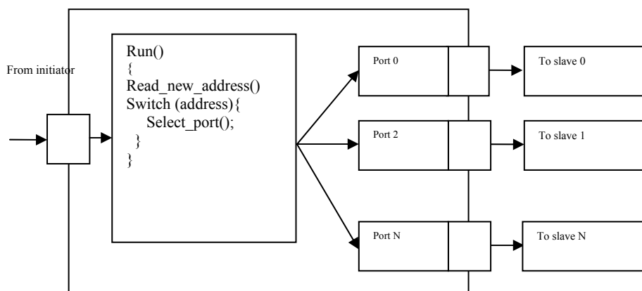
Figure 3. Router component
