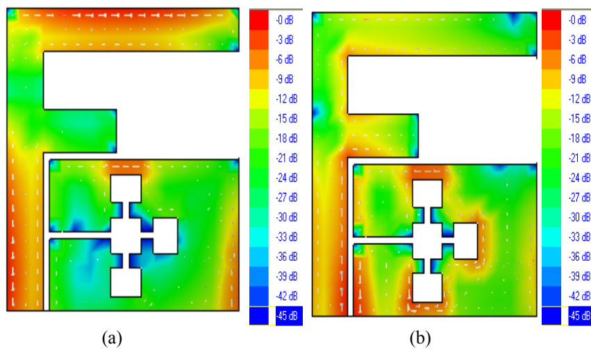
Figure 4. Current distribution of proposed antenna (a) 3.4GHz (b) 5.5GHz
