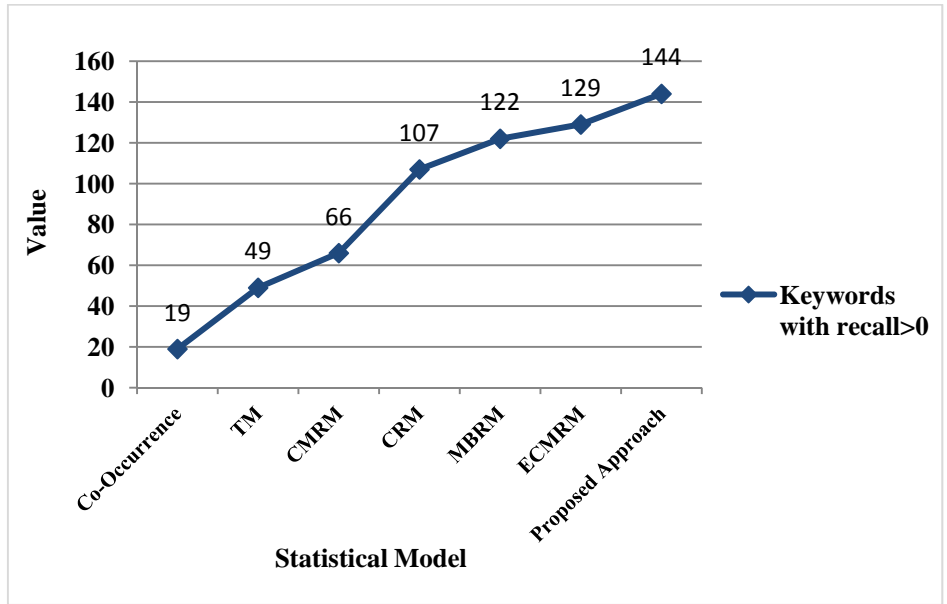
Figure 7. Keywords with recall>0 in some statistical models
