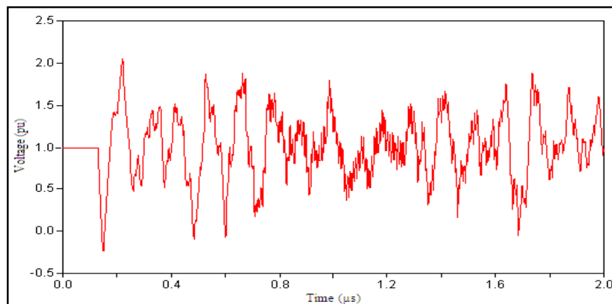
Figure 5. VFTO at Tr1 (Worst Case)
