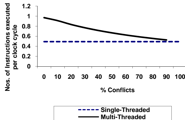
Figure 6. Performance with respect to dependencies among the threads
