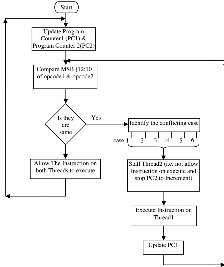
Figure 3. Flow Chart - Conflict Resolver
