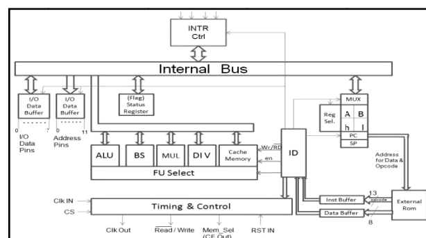
Figure 1. Architectural Diagram of Single Threaded Processor
