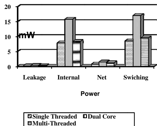
Figure 5. Power consumption in mW
