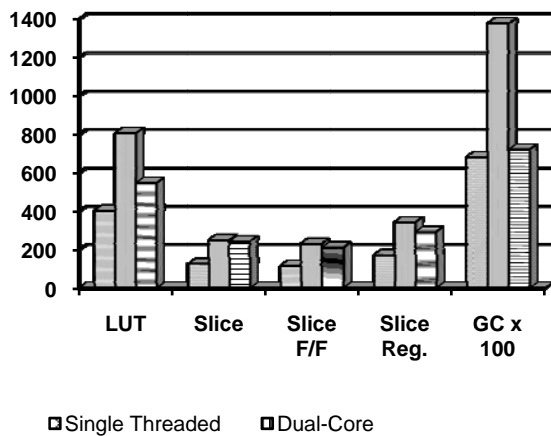
Figure 4. Area comparison in terms LUT, Slice, F/F, Registers and Gate count
