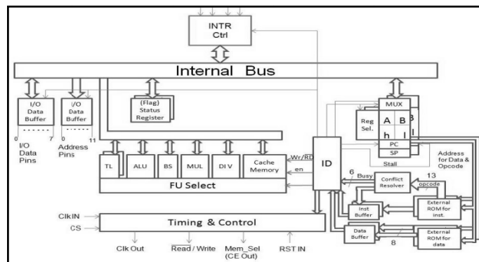
Figure 2. Architecture of Multi-Threaded Processor
