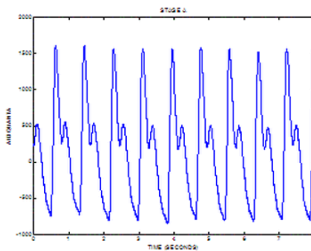
Figure 9. PPG signals from commercial heart rate monitor 2
