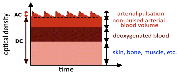
Figure 1. AC and DC components of fiber optic PPG
