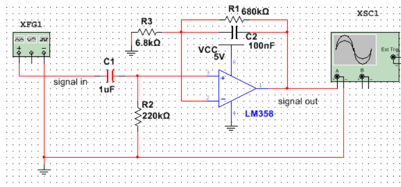
Figure 2. Passive high pass filter and active low pass filter
