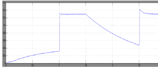
Figure 15. Capacitor Voltage
