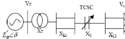
Figure 1. Diagram of one machine - infinity bus system
