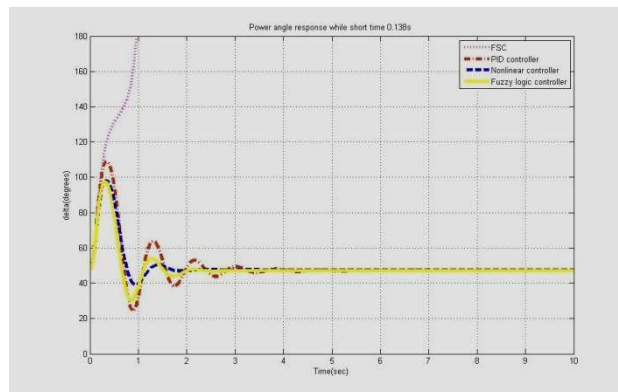
Figure 6. power angle response while short time 0.138s
