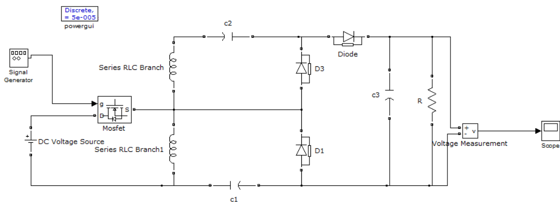
Figure 5. Simulation of Boost Converter using Matlab/Simulink
