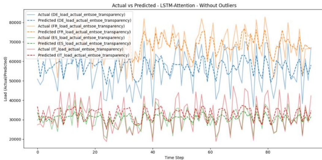
Figure 4. Load forecasting using LSTM without outliers removed
