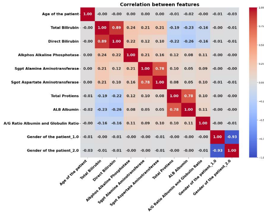
Figure 5. Correlation matrix between variables, highlighting relationships between liver function tests and demographic data. Strong correlations are evident among liver enzymes and proteins, with gender displaying a notable negative correlation between its binary categories. This matrix offers critical insights for precise liver function analysis
