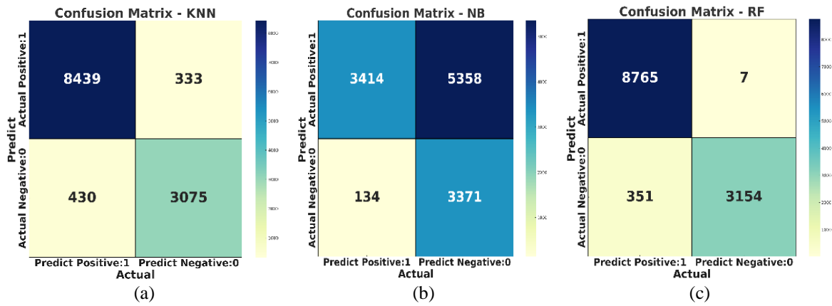
Figure 3. Confusion matrix for (a) KNN, (b) Gaussian NB, and (c) RF. KNN and Gaussian NB has higher false positive rates, while RF exhibits minimal false positives and negatives, resulting in a higher true positive count
