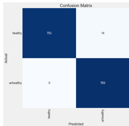
Figure 10. InceptionResNetV2's confusion matrix
