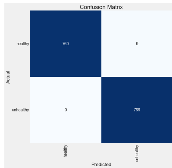
Figure 8. ResNet50's confusion matrix
