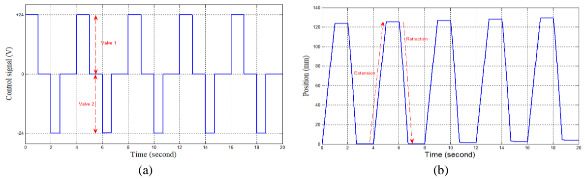
Figure 3. Plot of measured data: (a) input and (b) output
