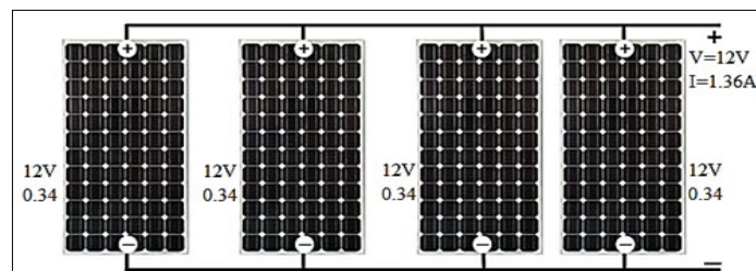
Figure 3. Four PV panels connected in parallel
