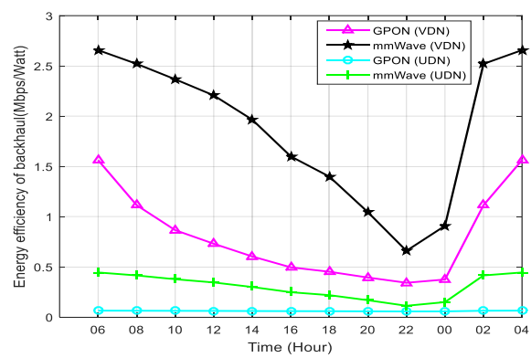
Figure 5. Graph of power consumption of PON and mmWave in VDN and UDN
