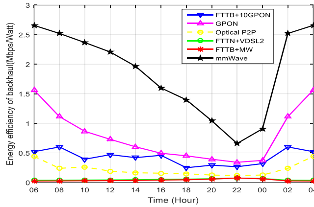
Figure 3. Graph of energy efficiency of the backhaul solutions
