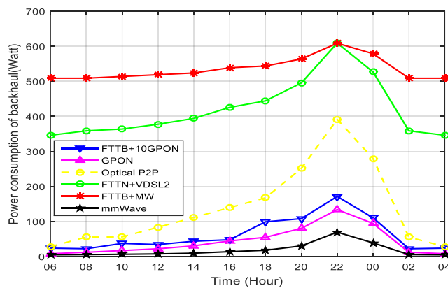
Figure 2. Graph of power consumption of the backhaul solutions
