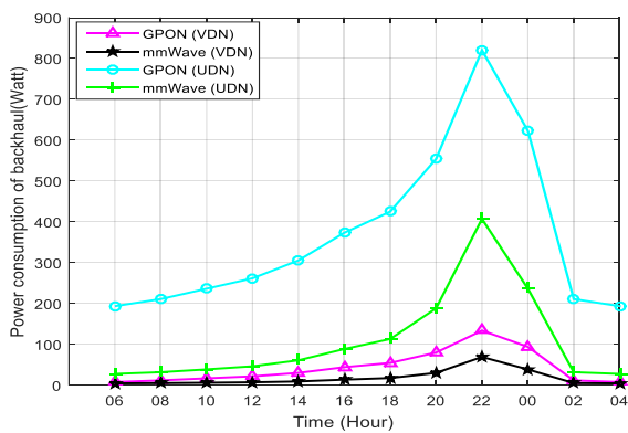
Figure 4. Graph of power consumption of PON and mmWave in VDN and UDN
