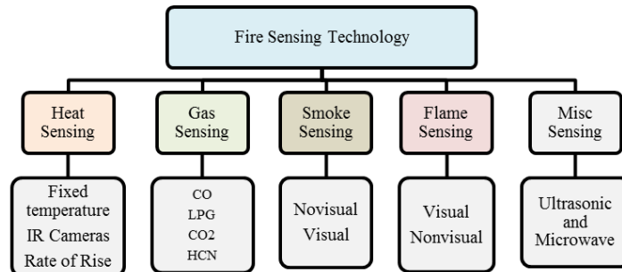
Figure 1. Fire sensing technologies[31]
