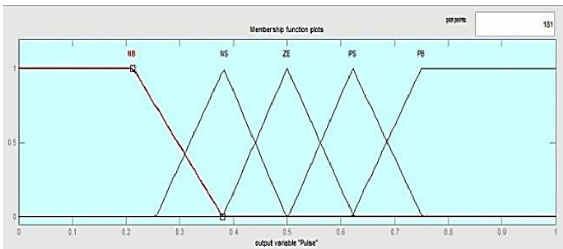
Figure 9. Output membership function of duty cycle
