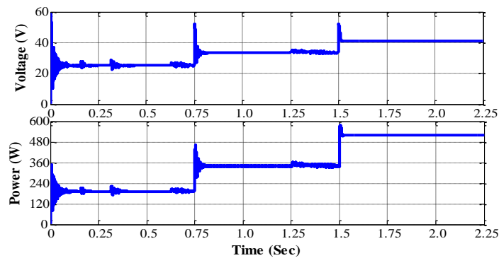
Figure 17. Wind system output voltage and power
