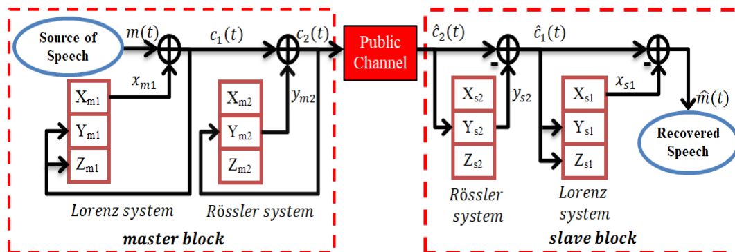
Figure 3. Double masking proposed system under the AWGN channel
