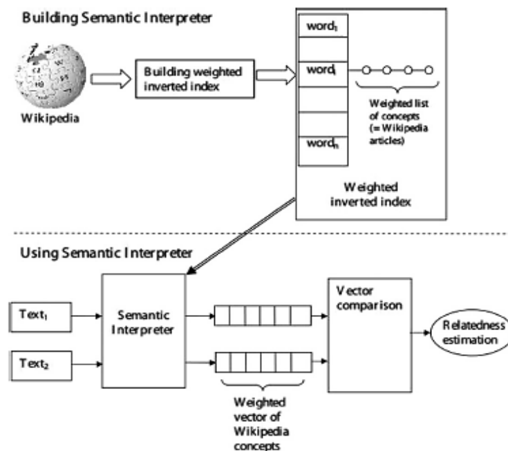
Figure 1. Explicit semantic analysis ESA system
