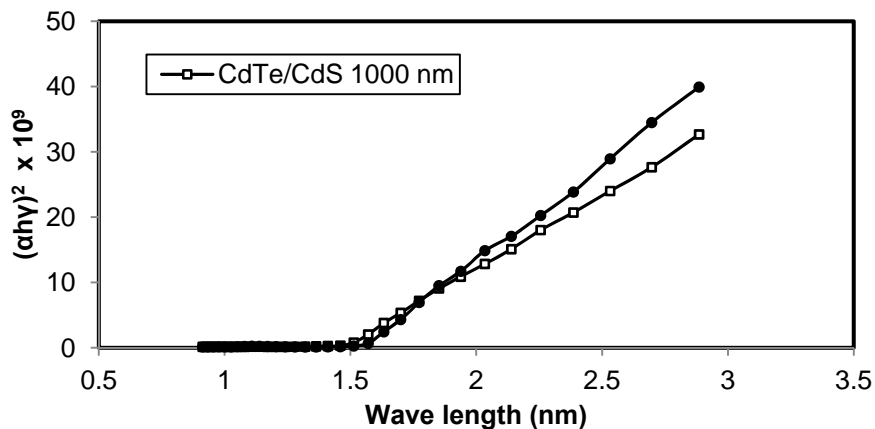
Figure 6. (\alpha h\nu)^2 vs photon energy ( h\nu ) plot of CdS/CdTe thin films
