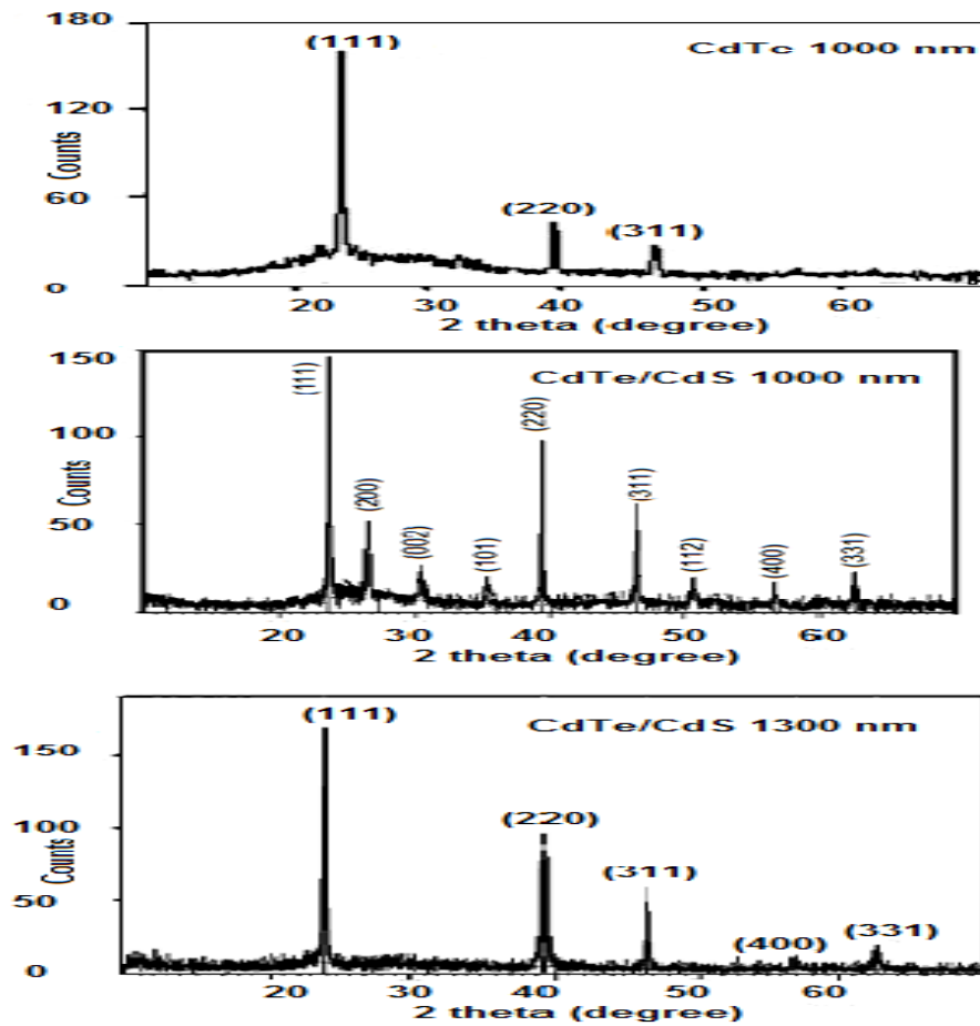
Figure 1. XRD spectra of (a) CdTe 1000 nm (b) CdTe/CdS 1000 nm (c) CdTe/CdS 1300 nm
