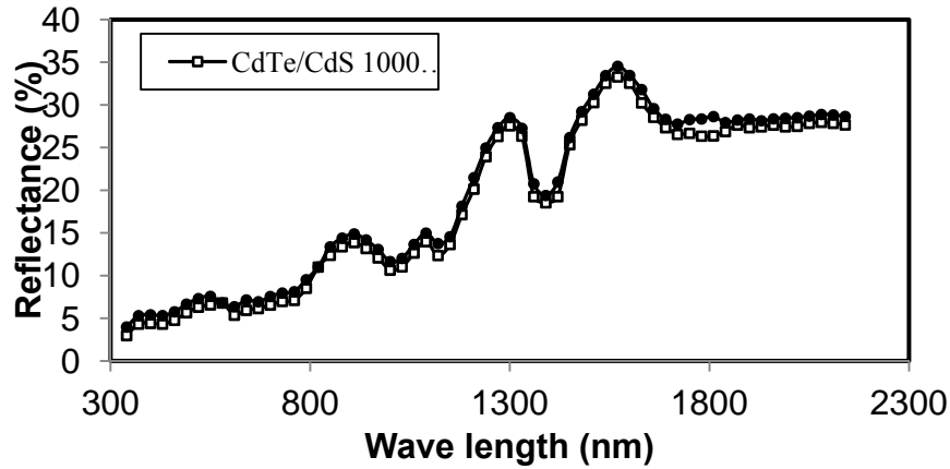
Figure 4. Reflectance variation of CdTe thin films
