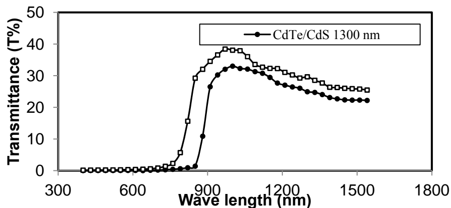
Figure 3. Transmittance variation of CdTe thin films with wavelength
