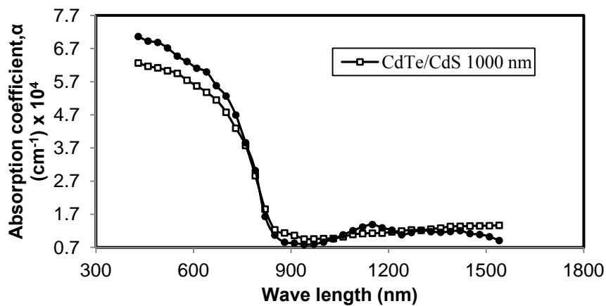
Figure 5. Absorption coefficient variation of CdTe thin films
