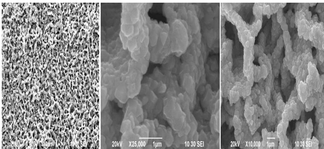
Figure 2. SEM image of CdTe thin film of thickness 1000 nm deposited on CdS thin film with magnification X25000
