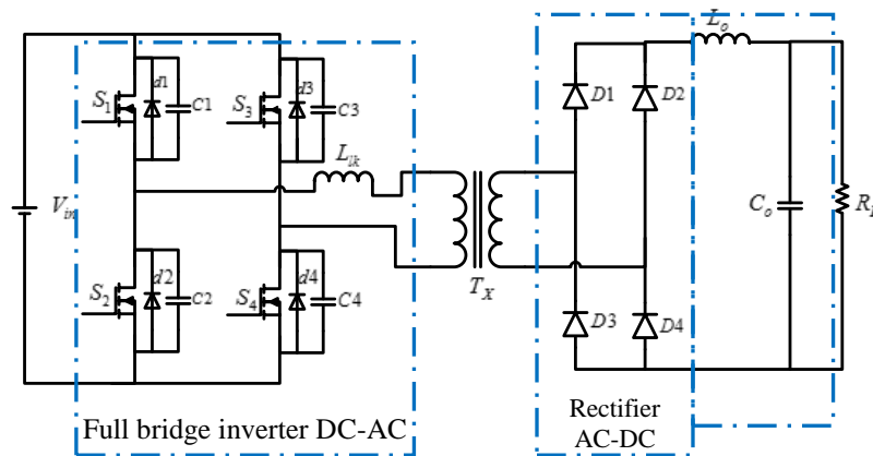
Figure 1. Full bridge DC-DC converter
