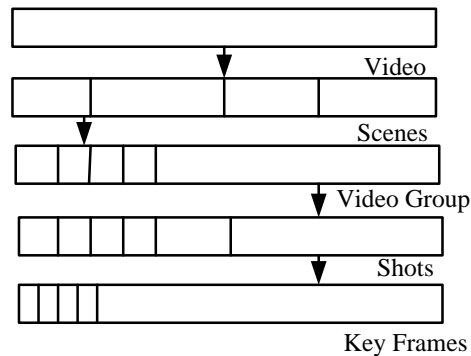
Figure 1. Video Hierarchy
