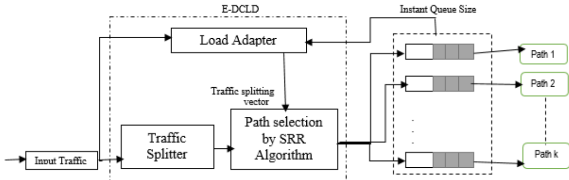
Figure 3. Proposed architecture in wireless sensor applications
